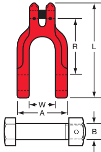
Crosby Trawlex® Dog Shackle KDL
