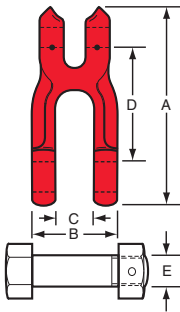
Crosby Trawlex® Narrow Jaw Shackle KDN
