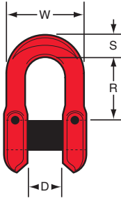
Crosby Trawlex® 'D' Shackle TXRC
